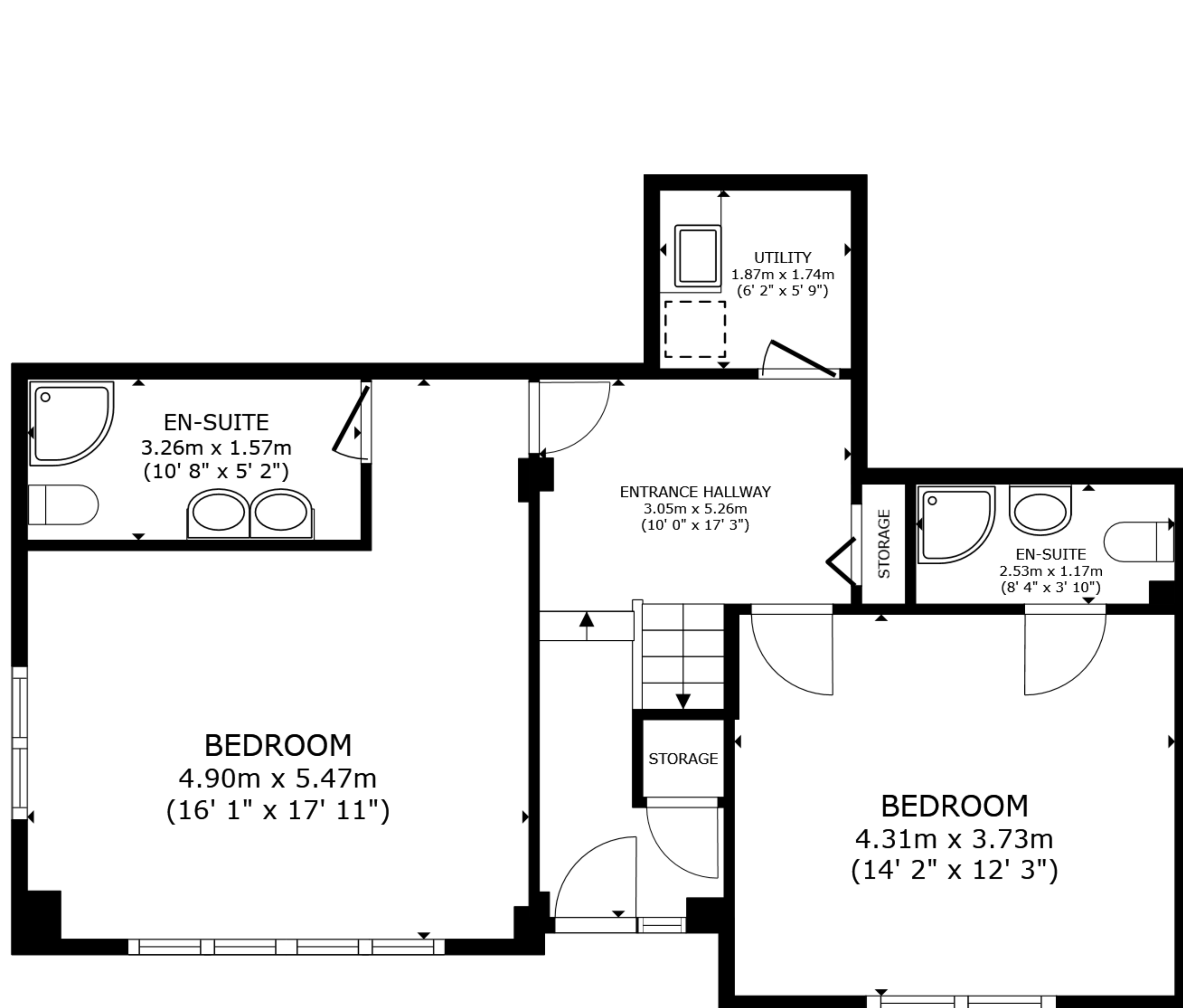
FLOOR 1
